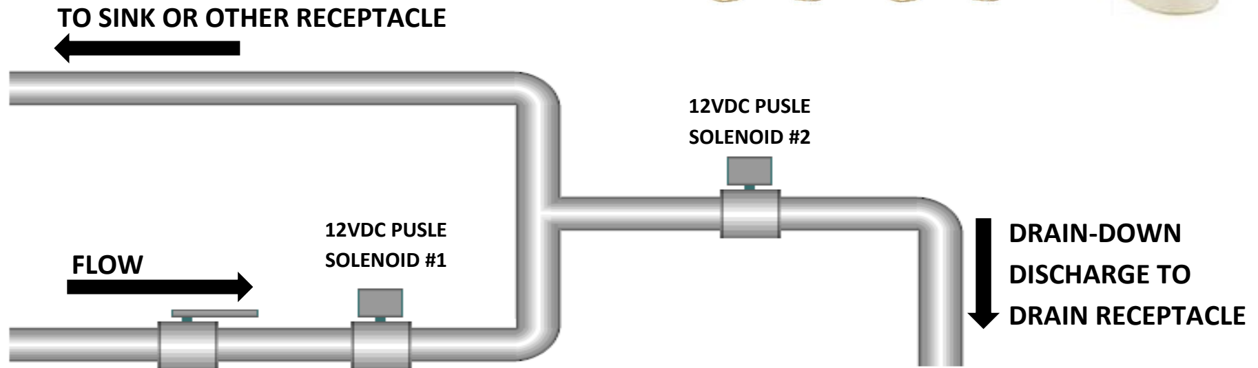
PIPING ILLUSTRATION REPRESENTING THE OPERATION AND FUNCTION OF THE SOLENOIDS
